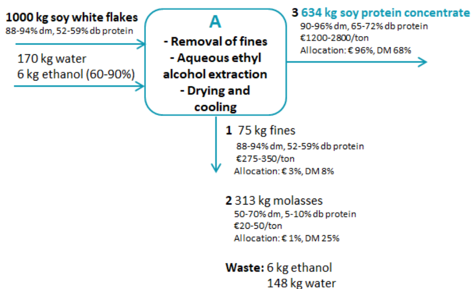
Figure 15: Soy protein-concentrate production process (Van Veghel, 2017).
