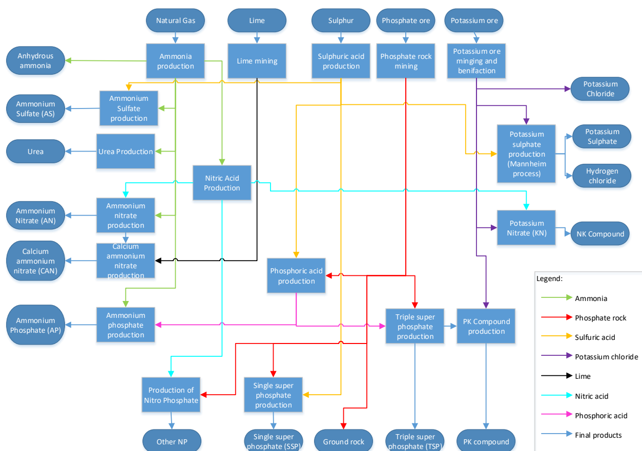
Figure 20: Product flow diagram for fertilizer production. The colored lines indicate specific intermediate flows (see legend). Raw materials are listed on the top of the figure, N fertilizers are listed on the left, P fertilizers on the bottom, K fertilizers on the right. Figure based on description in Kongshaug (1998).
