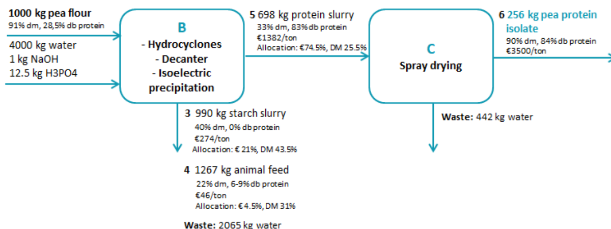
Figure 19: Pea protein-isolate production process (Van Veghel, 2017).
