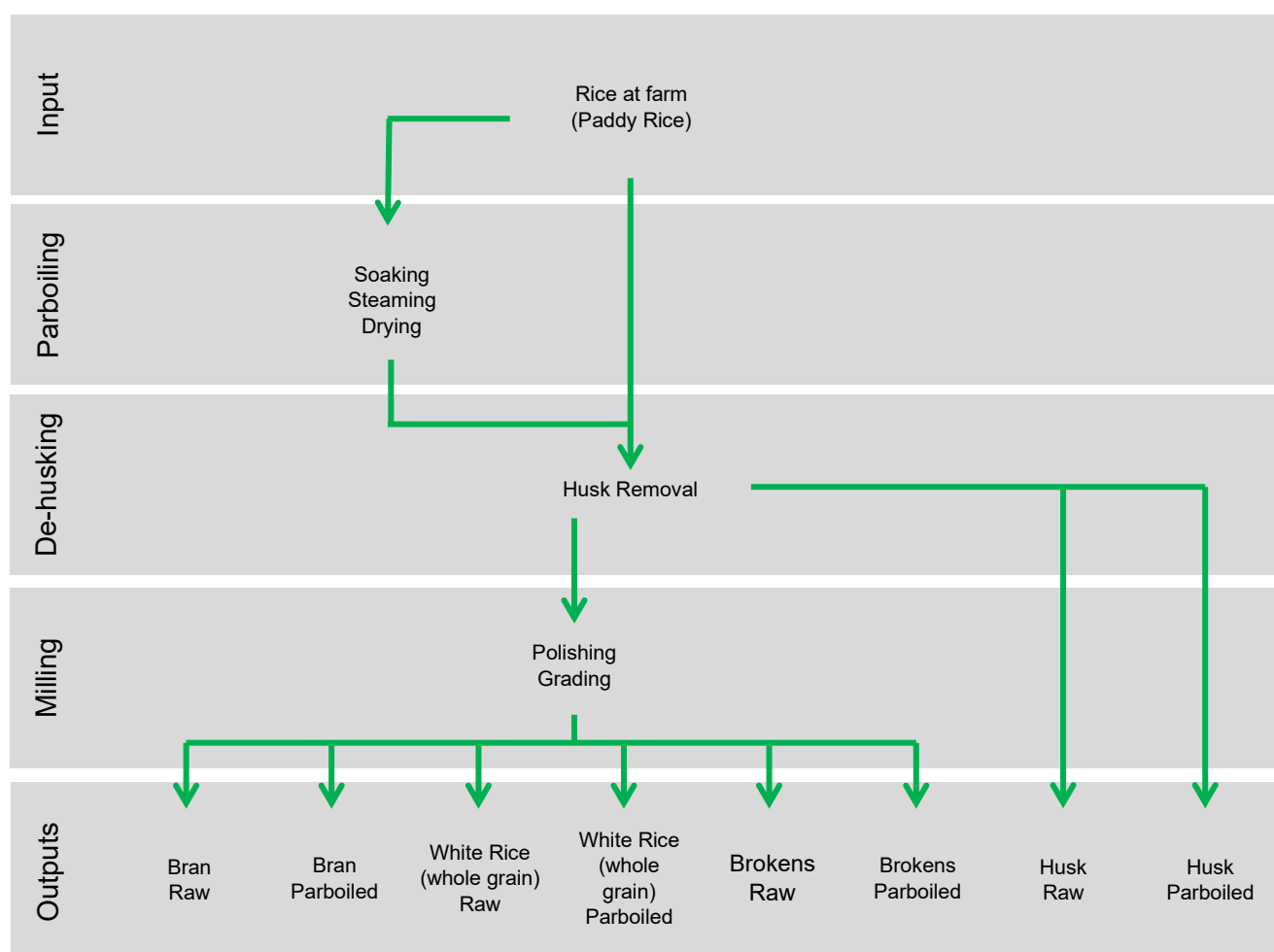
Figure 13: Diagram describing the process of production of white rice, rice husks, rice bran, and rice brokens from a rice dry milling process in China.
