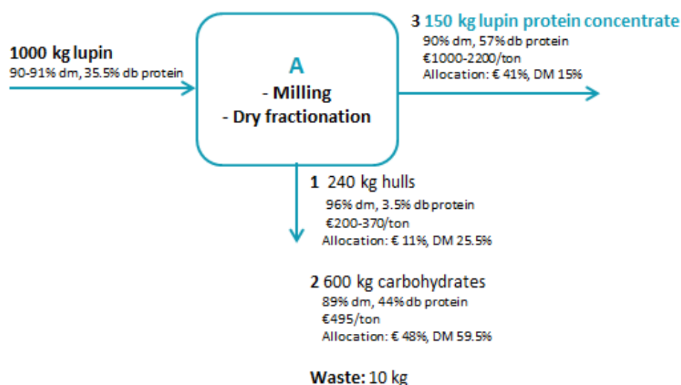
Figure 14: Lupin protein-concentrate production process (Van Veghel, 2017).
