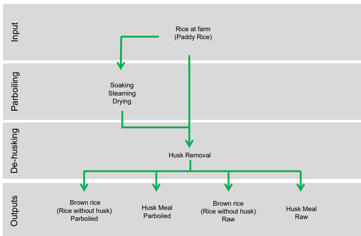
Figure 12: Diagram describing the process of production of rice without husks and rice husks from a rice dry milling process.
