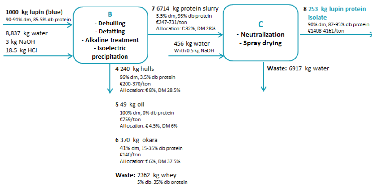
Figure 18: Lupin protein-isolate production process (Van Veghel, 2017).
