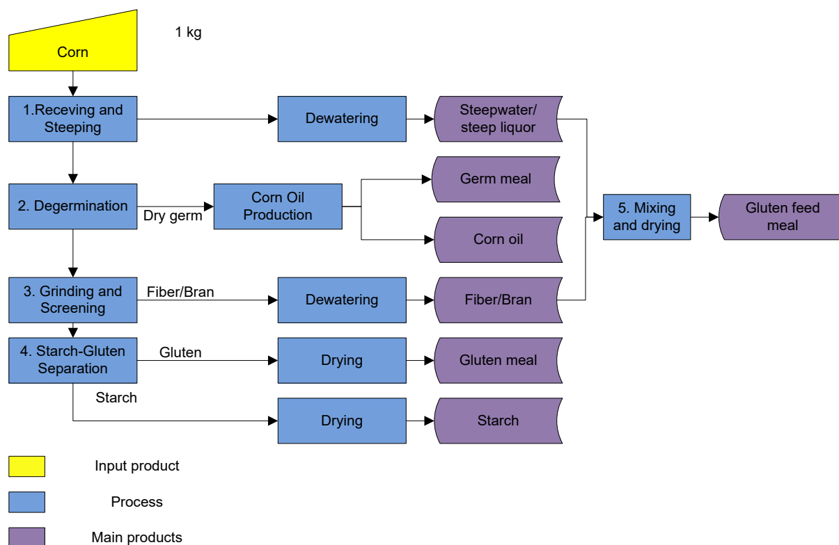
Figure 11: Wet milling of maize (van Zeist et al., 2012f).
