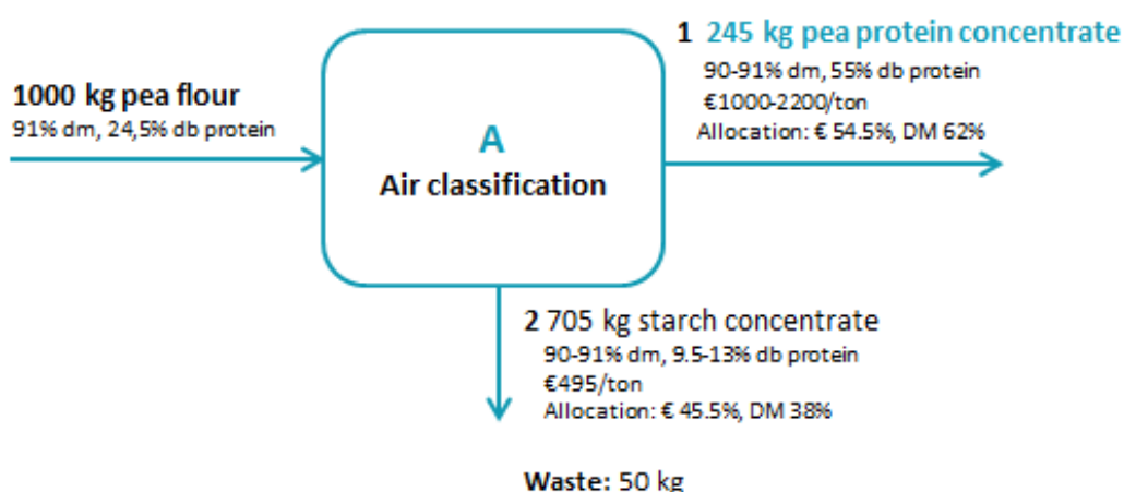
Figure 16: Pea protein-concentrate production process (Van Veghel, 2017).
