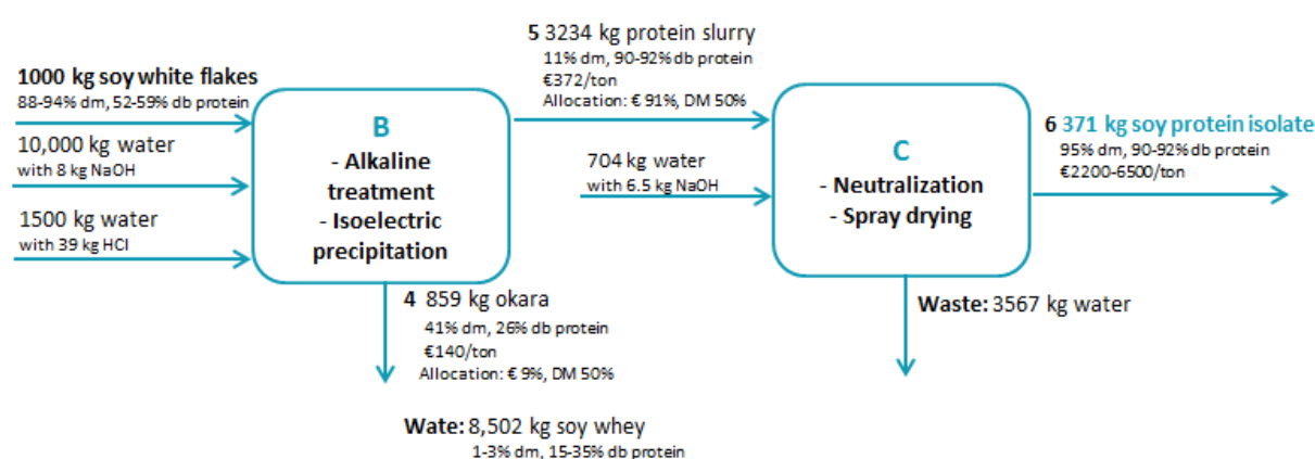
Figure 17: Soy protein-isolate production process (Van Veghel, 2017).
